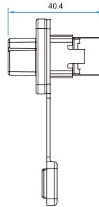
插座 SX (外型尺寸图) SX socket (dimensions figure)
