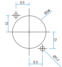
安装开孔图 Installation hole figure
