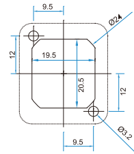
安装开孔图 Installation hole figure
