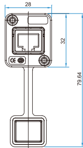
插座 SX (外型尺寸图) SX socket (dimensions figure)
